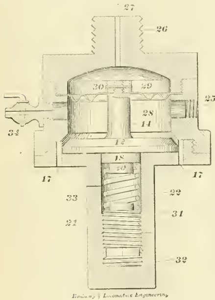
PRESSURE RETAINING AND RECHARGING DEVICE.
